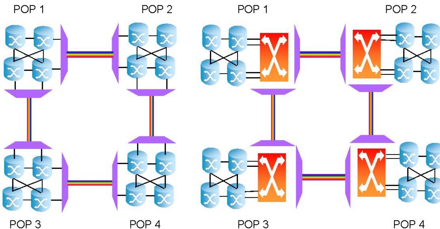
Architecture A: Routers connected via DWDM links
