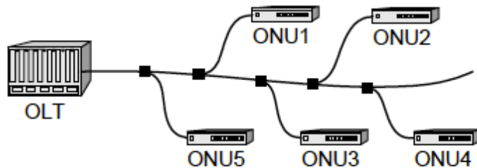
(b) Bus topology (using 1:2 tap couplers)
