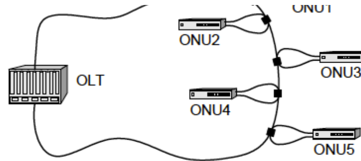
(c) Ring topology (using 2x2 tap couplers)
